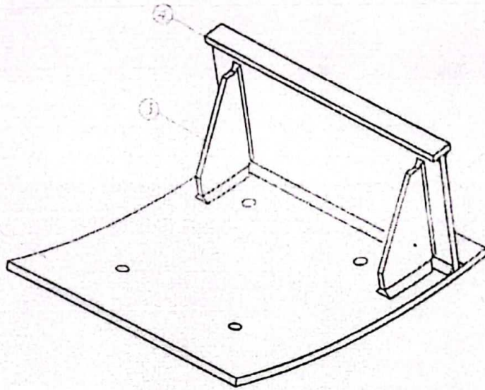
3D assembly view SCALE 1:5
