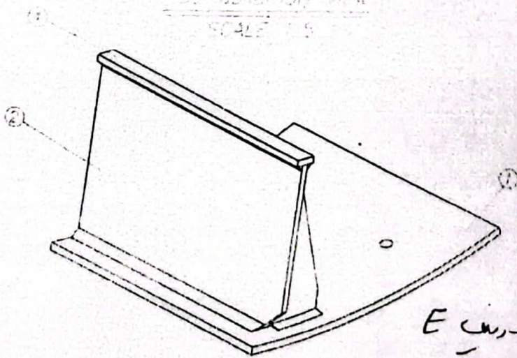
PERSPECTIVE VIEW SCALE: 1:5
