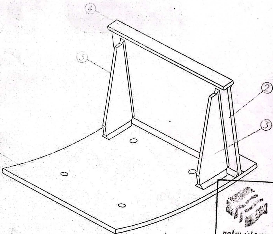
3D assembly view SCALE 1:5
