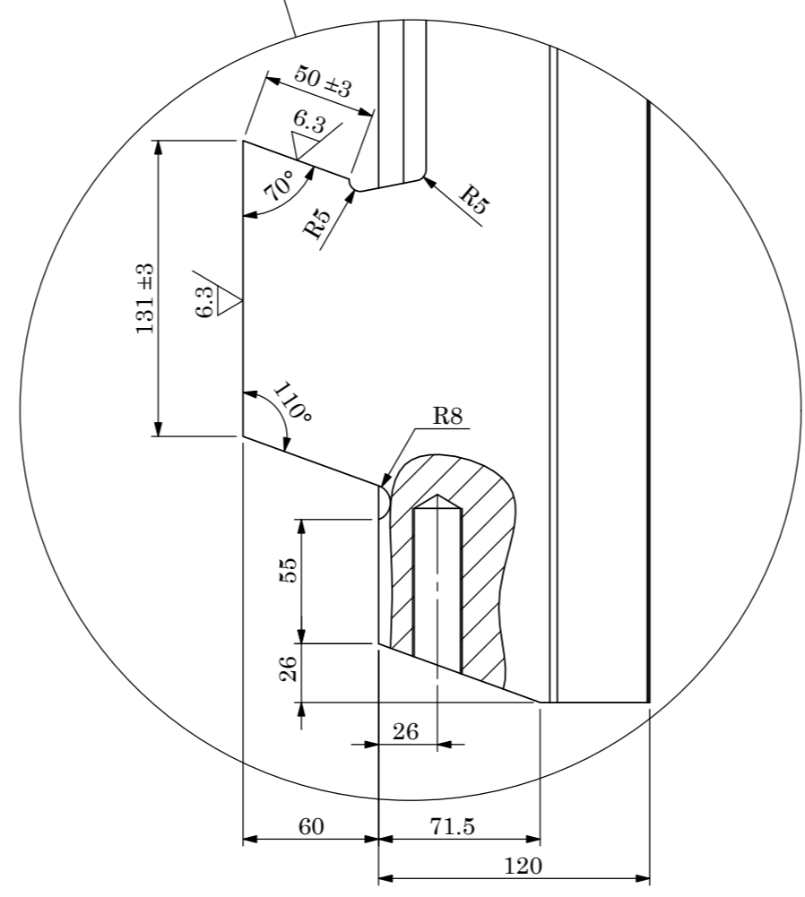
DETAIL A SCALE 1 : 3
