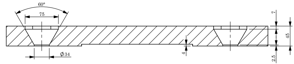
SECTION P-P
