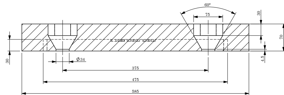
SECTION S-S
