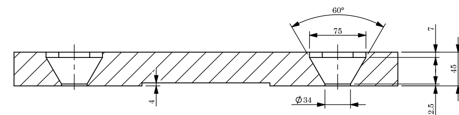
SECTION K-K
