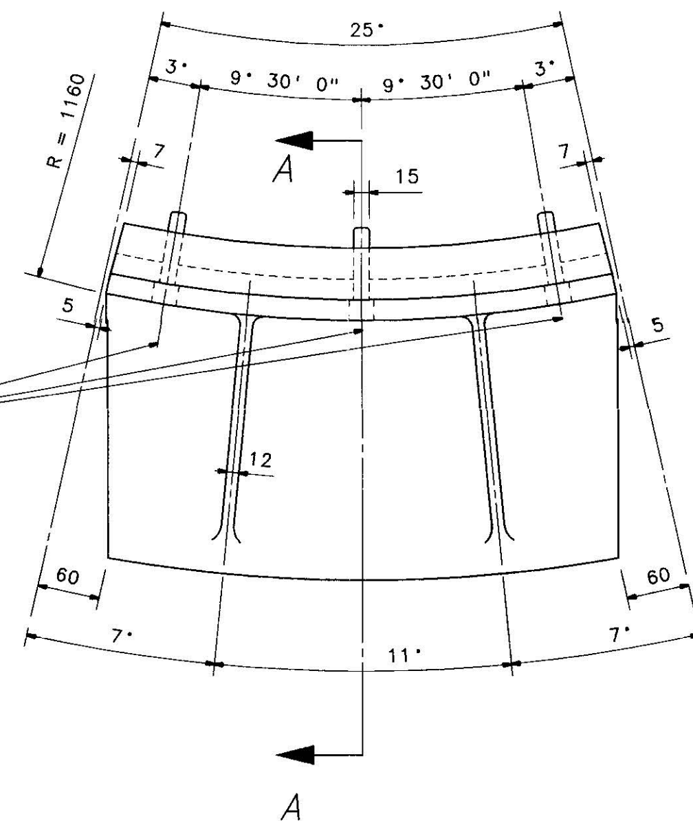
DETAIL OF ONE SECTOR SCALE 1/5
